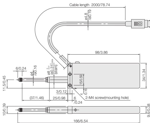
DL330B
